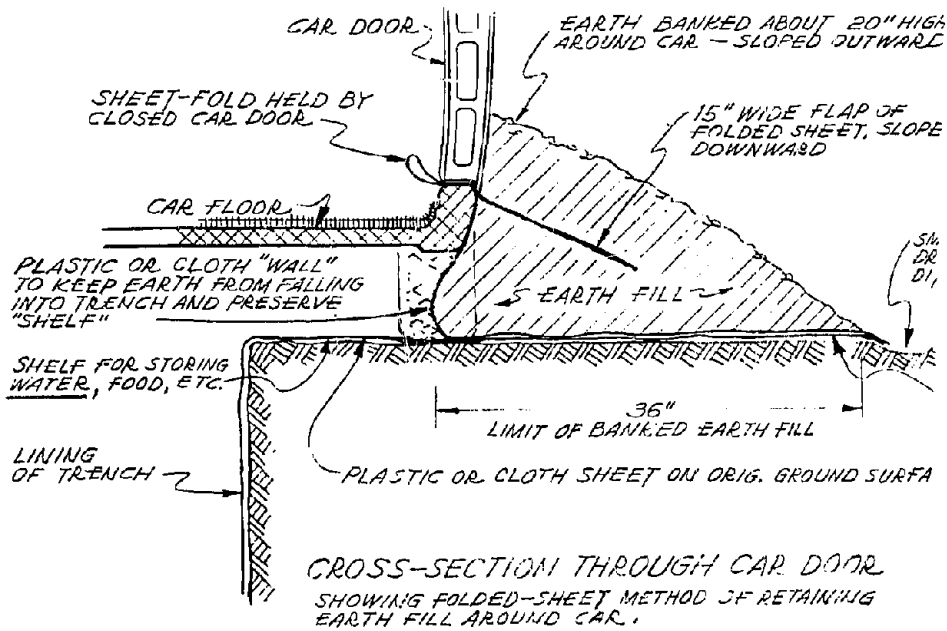
Fig. A-13.3. Car-Over-Trench Shelter, Front View and Cross Section.
